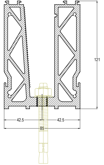
A - A KESİTİ A - A SECTION
