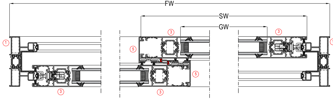
NORMAL SÜRME SİSTEM NORMAL SLIDING SYSTEM
